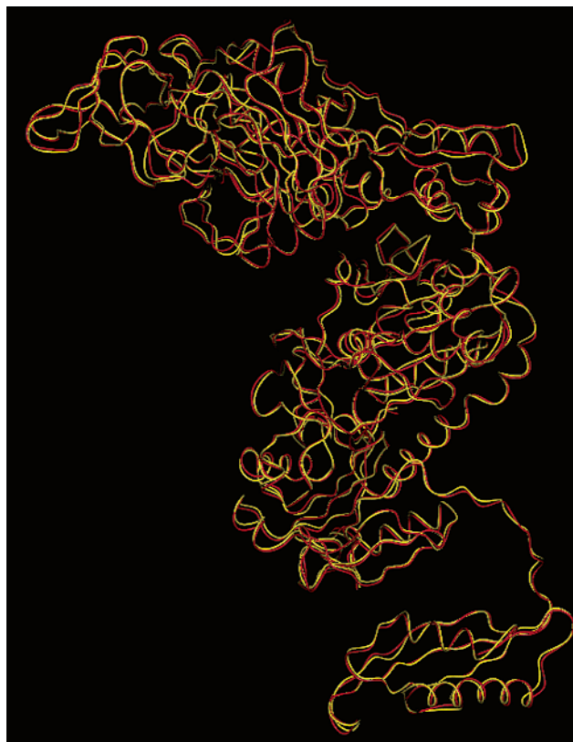
Figure 1. Comparison of crystal structure without ligand (No/PheRS, IPYS) in red with the force field-minimized structure in yellow. CRMS = 0.8 Å.
