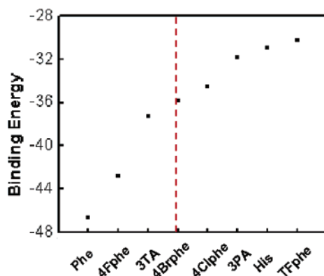
Figure 5. Calculated binding energies for analogues of Phe in PheRS. The analogues are shown in Scheme 1. The analogues to the left of the broken line have been observed experimentally to serve as phenylalanine surrogates in wild-type E. coli cells; those to the right have not. The abbreviations in the figure for the Phe analogues are phenylalanine (Phe), p -fluorophenylalanine (4Fphe), p -chlorophenylalanine (4Clphe), p -bromophenylalanine (4Brphe), 2,4,6-trifluorophenylalanine (TFphe), 3-thienylalanine (3TA), 3-pyrrolylalanine (3PA), and histidine (His).
