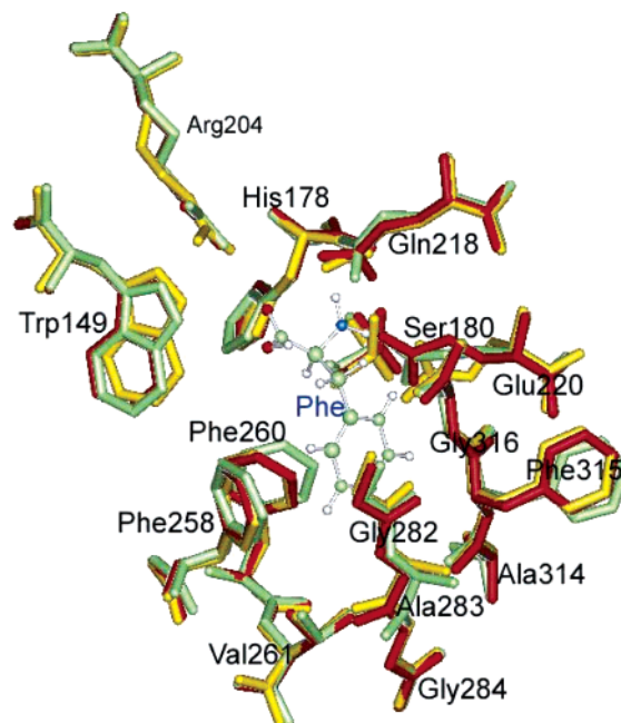
Figure 3. Comparison of binding pocket for PheRS from (a) No/PheRS, ligand-free crystal structure (red) of (b) minimized structure from No/PheRS (yellow), and (c) the Phe/PheRS crystal structure (1B70) (green).
