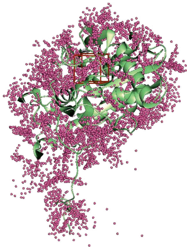
Figure 2. \alpha -Subunit of T. thermophilus PheRS from the crystal structure (No/PheRS, 1PYS). The dots show the potential binding sites, and the box shows the binding region used for HierDock.
