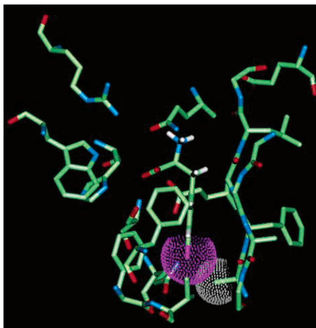
Figure 6. The van der Waals surface (bromine atom surface shown in pink) of bromophenylalanine clashing with the vdW surface of the side chain of Ala314.
