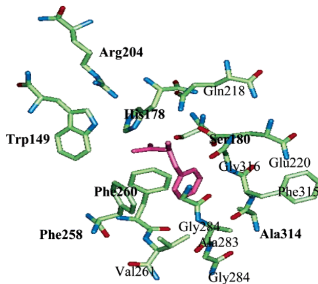
Figure 4. Predicted binding site of Phe in PheRS from applying HierDock to No/PheRS. The predicted position of the Phe is shown as pink sticks.
