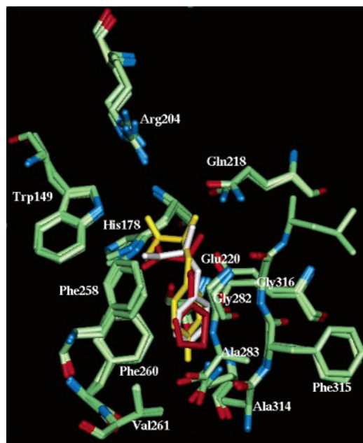
Figure 7. Comparison of binding pocket for phenylalanine (white) to that of p -fluorophenylalanine (yellow) and 3-thienylalanine (red).
